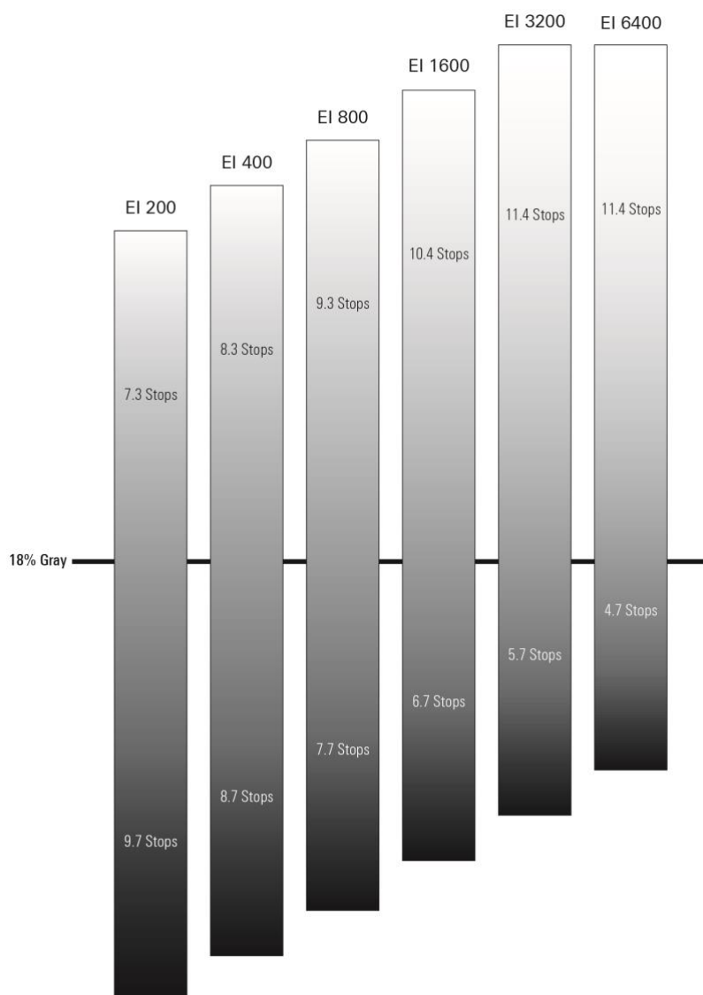
Distribution of dynamic range at a given ISO rating for ALEXA 35/ALEXA 35 Xtreme (regular mode).
