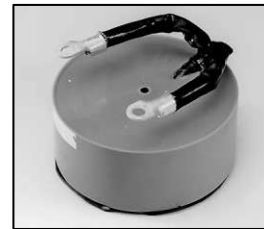
L4.82385.E HF-choke 230 V / 130 A HF-Drossel 230 V / 130 A
