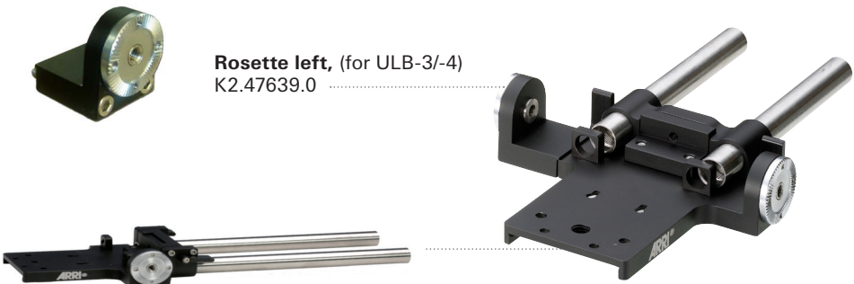
Universal Lightweight Support ULB-4 incl. rods, K2.47651.0
