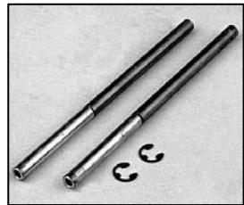
L4.79647.E Focus support rods Gleitstange
