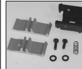
L4.80747.E Door catch set for rear loader versions Schnapphaken-Set für Hecklader Version
